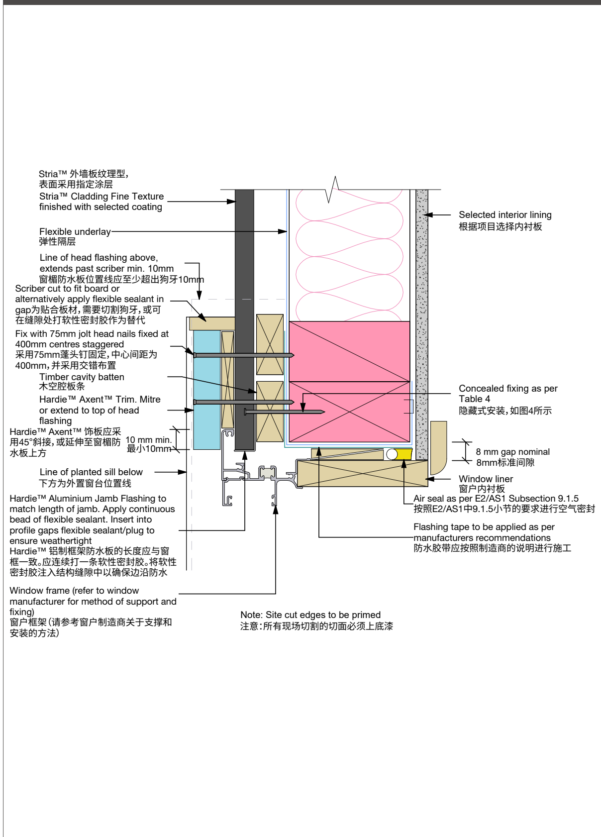
Figure 24: Window jamb with facings | 图24: 带饰面的窗框
