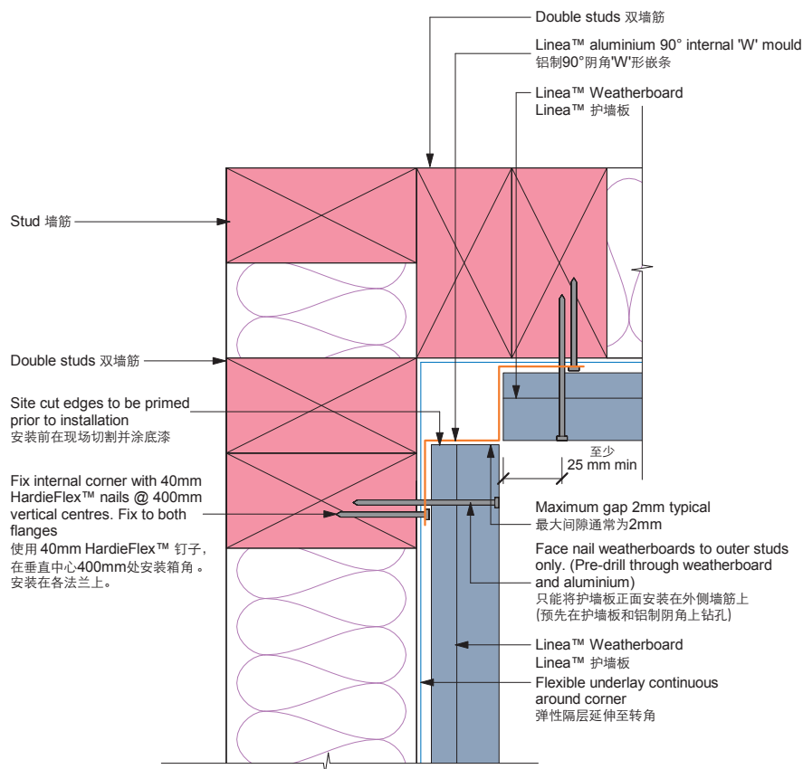
Figure 9: Internal aluminium corner | 图 9: 铝制阴角
