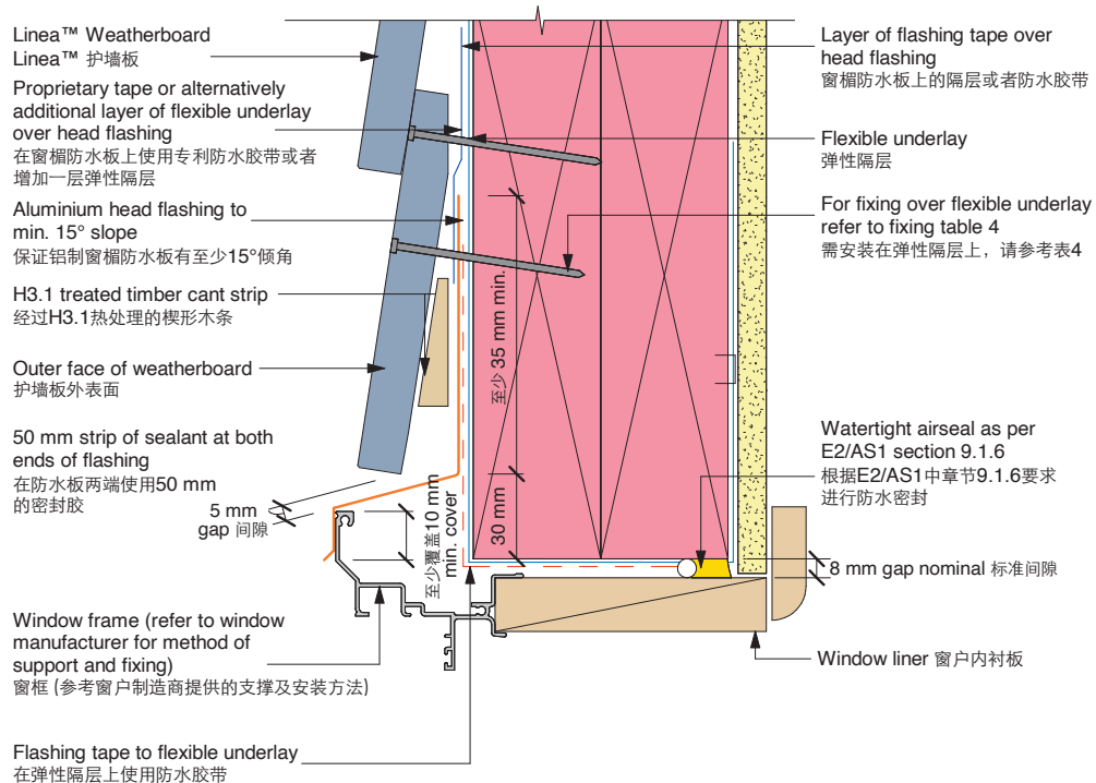
Figure 14: Window head | 图 14: 窗楣
