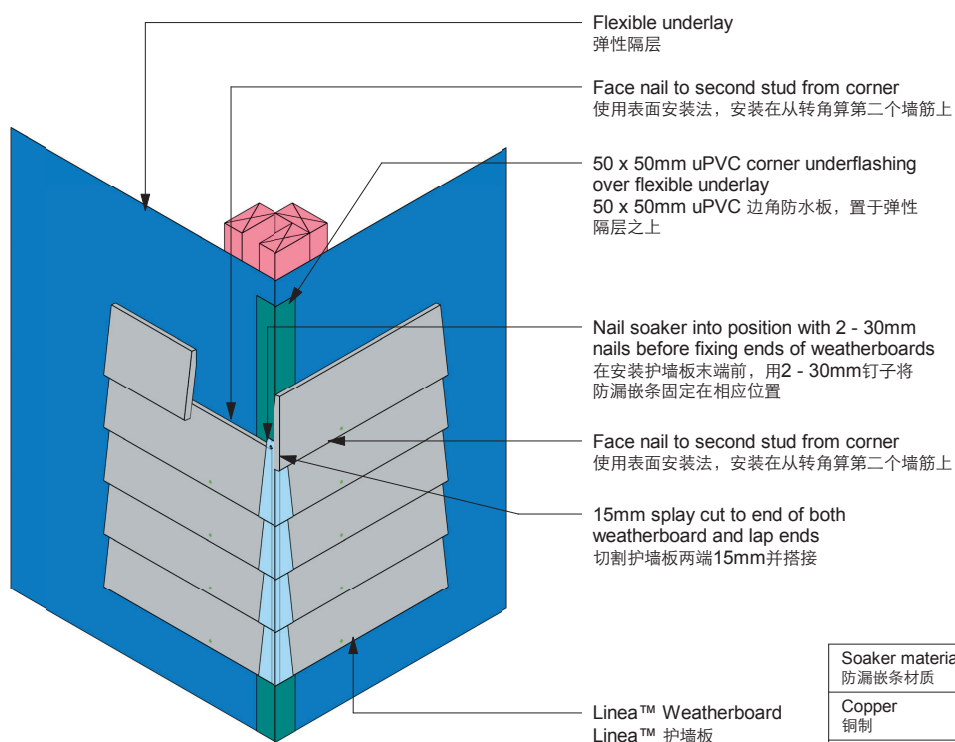
Figure 5: External corner soaker | 图 5: 阳角防漏嵌条
