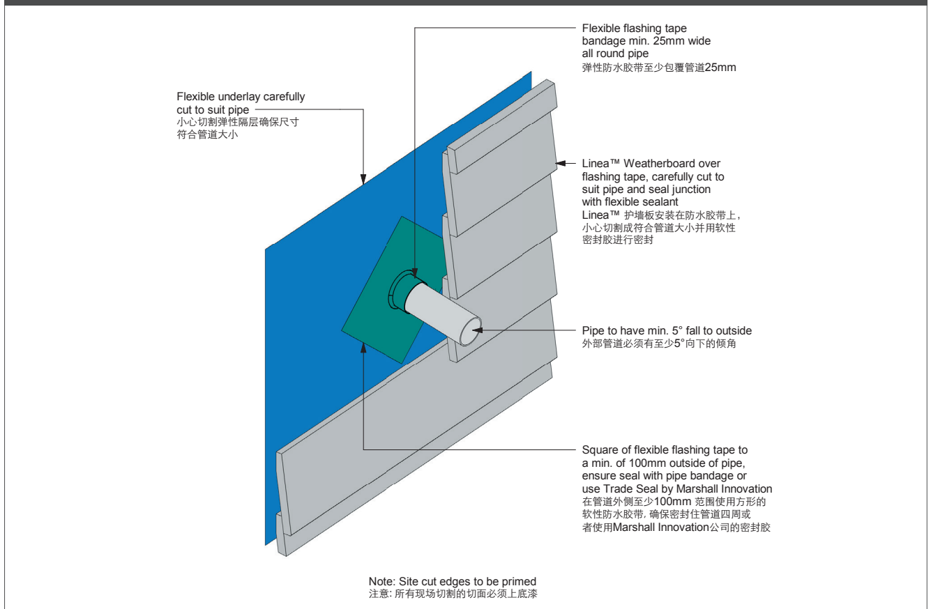
Figure 20: Pipe penetration | 图 20: 管道穿透
