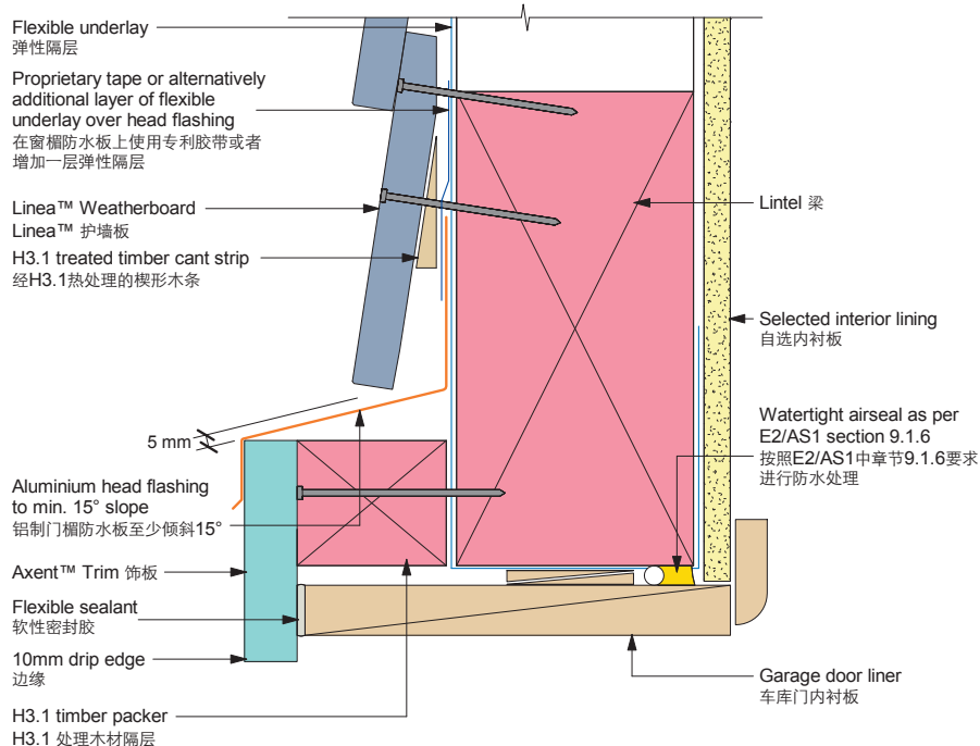
Figure 24: Garage door head | 图 24: 车库门楣
