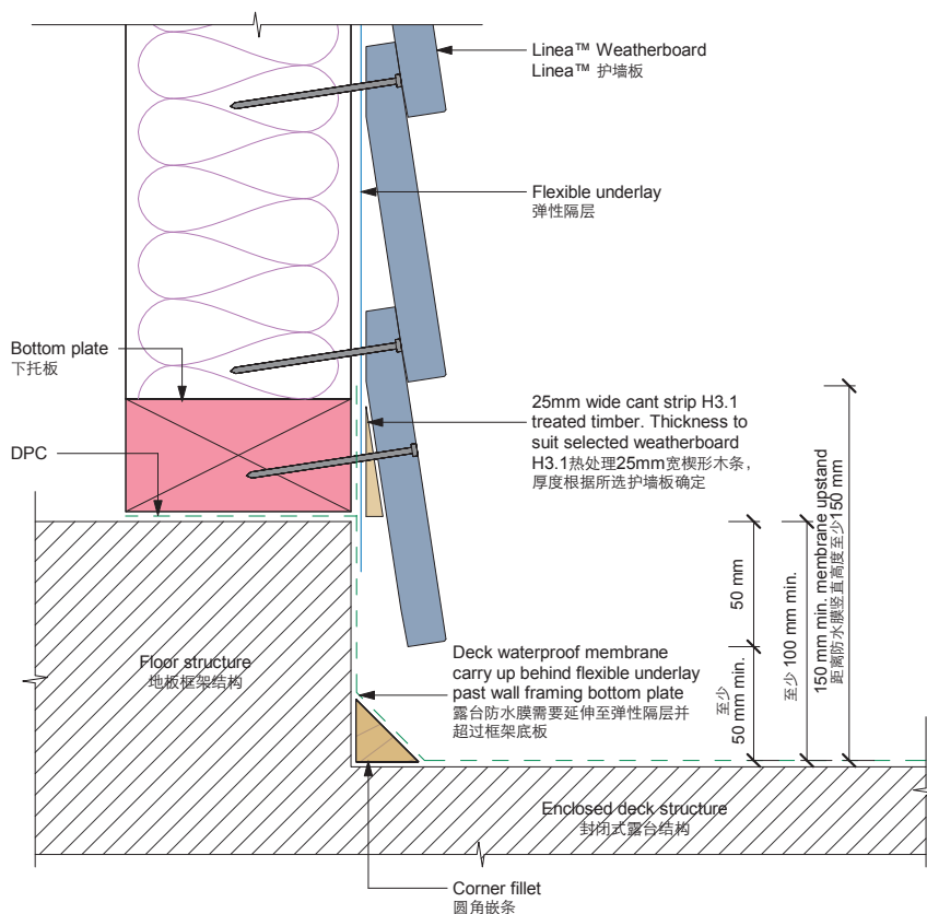
Figure 3: Enclosed deck | 图 3: 封闭式露台
