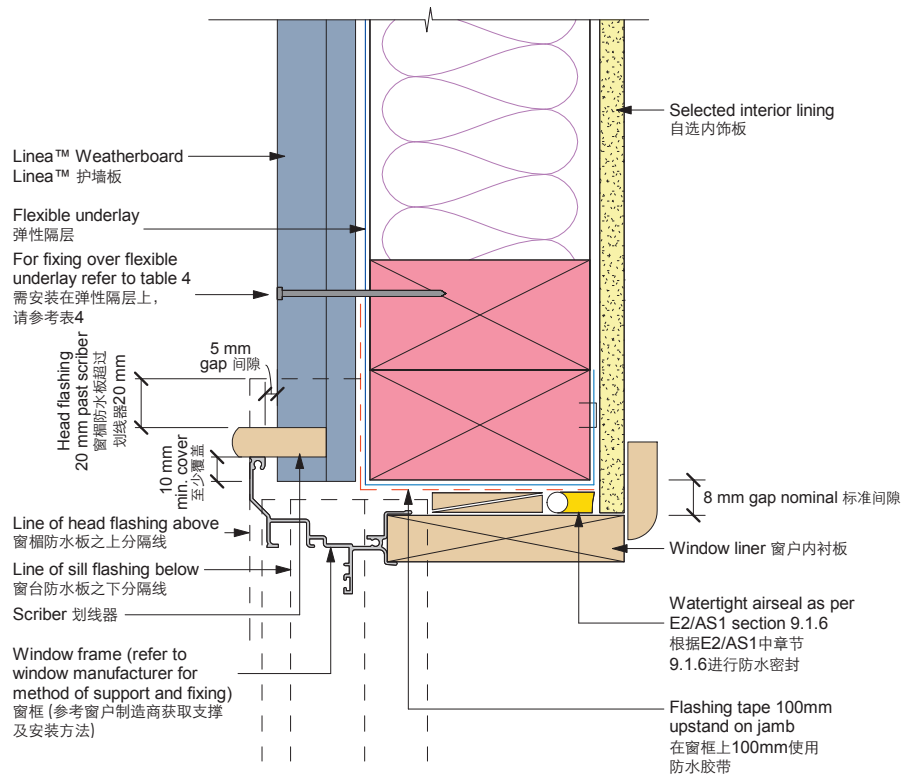
Figure 15: Window jamb | 图 15: 窗框
