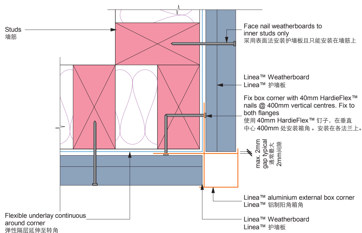
Figure 6: External aluminium box corner | 图 6: 铝制阳角箱角
