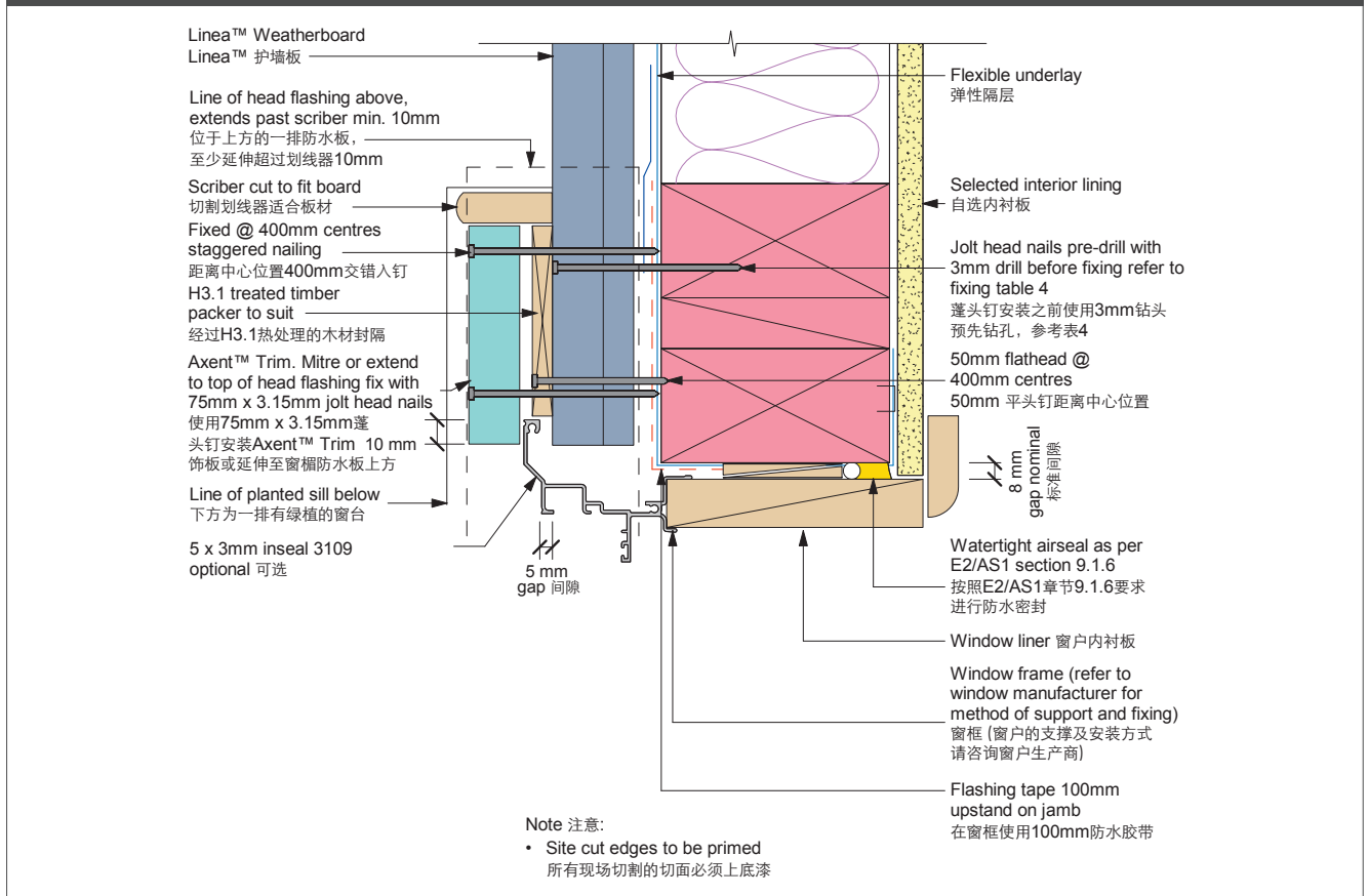
Figure 19: Window jamb with facing | 图 19: 带有装饰板的窗框
