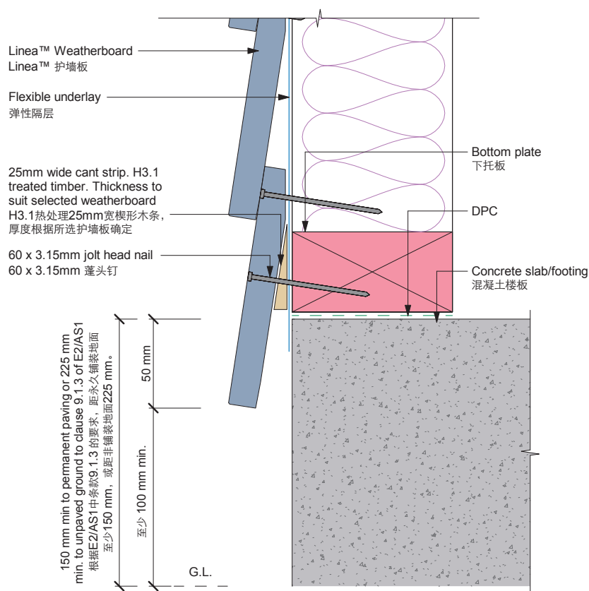
Figure 2: Direct fix foundation detail and soffit detail | 图 2: 直接安装法地基详图和拱腹详图
