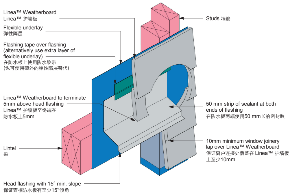
Figure 16: Head flashing termination | 图 16: 窗楣防水板终端
