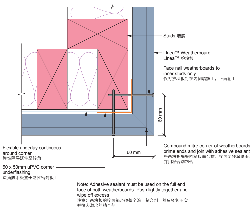
Figure 8: External mitre corner | 图 8: 阳角斜接边角
