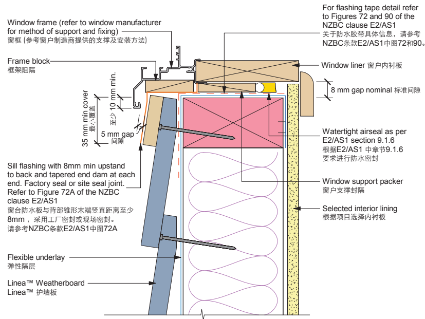
Figure 13: Window sill | 图 13: 窗台
