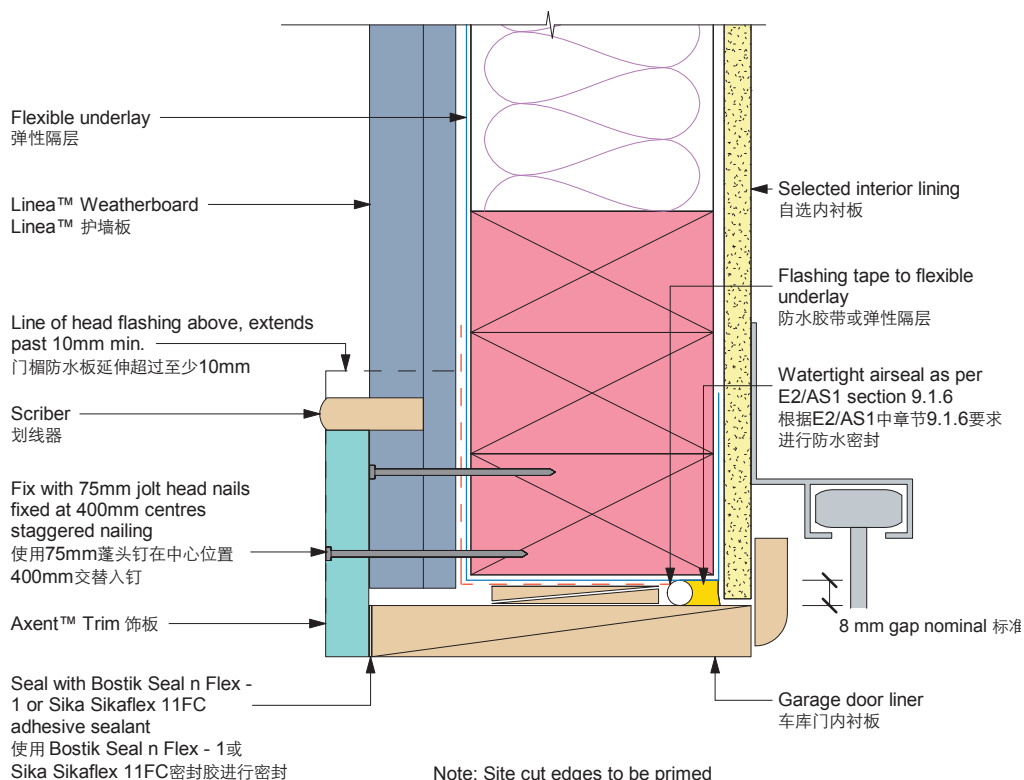
Figure 25: Garage door jamb | 图 25: 车库门框
