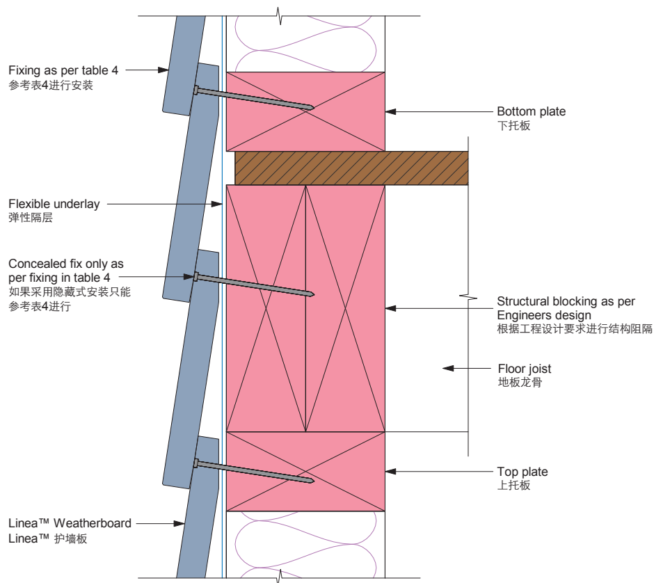
Figure 21: Continous cladding over joist | 图 21: 龙骨上方的连续墙面
